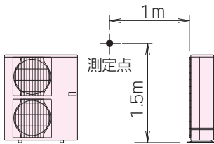
KM-5A
