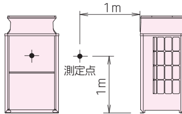
KM-8A/10A
