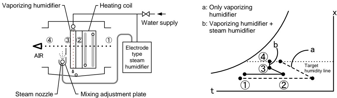
Figure 9-3. Hybrid humidification
