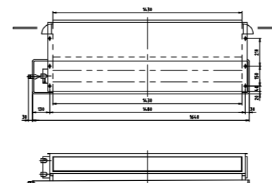
HSR6-1200ZF
