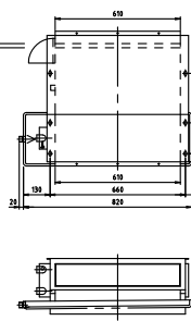
HSR6-300ZFP2
