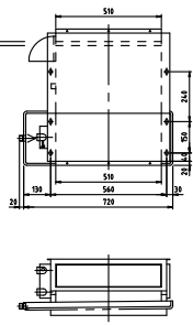
HSR6-200ZFP2
