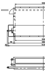
HSR6-800ZFP2
